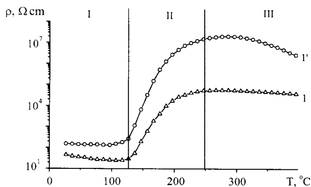
Fig. 7 Resistivity ( \rho ) of the PTCR ceramics ( \text{Ba}_x\text{Y}_{1-x}\text{TiO}_3 (1); ( \text{Ba}_x\text{Y}_{1-x}\text{TiO}_3 + 0.006 \text{ mol\% Mn} ) (1') versus temperature. I, II and III are the ranges with different character of dependences \rho(T)
