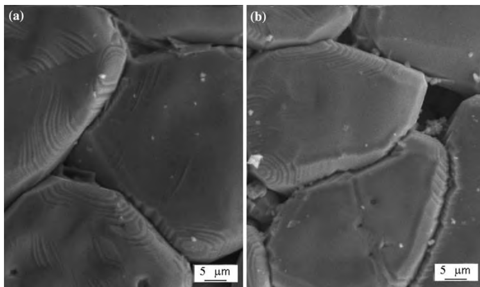
Fig. 6 Microstructure of the PTCR ceramics ( \text{Ba}_{0.996}\text{Y}_{0.004}\text{TiO}_3 (a); ( \text{Ba}_{0.996}\text{Y}_{0.004}\text{TiO}_3 + 0.006 \text{ mol\% Mn} ) (b). Scale bar = 10 \mu\text{m}
