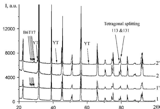
Fig. 2 Diffractograms of yttrium-doped barium titanate with the nominal compositions \text{Ba}_{0.99}\text{Y}_{0.01}\text{Ti}_{0.99}^{4+}\text{Ti}_{0.01}^{3+}\text{O}_3 (1, 1') and \text{Ba}_{0.975}\text{Y}_{0.025}\text{Ti}_{0.975}^{4+}\text{Ti}_{0.025}^{3+}\text{O}_3 (2, 2') after sintering in reducing atmosphere, \text{P}_{\text{O}_2} = 10^{-4} Pa (1, 2) and after oxidation in air for 20 h at 1,150 °C (1', 2'): BT = \text{BaTiO}_3 , \text{B}_6\text{Ti}_{17} = \text{Ba}_6\text{Ti}_{17}\text{O}_{40} , YT = \text{Y}_2\text{Ti}_2\text{O}_7
