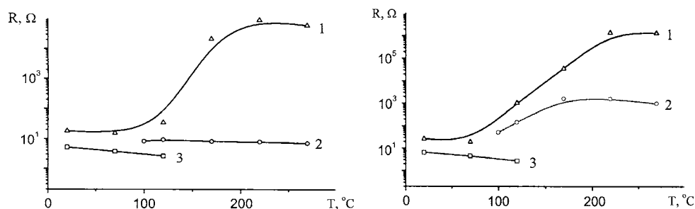
Fig. 8 Resistance of grain boundary (1), outer layer (2) and grain (3) of PTCR ceramics ( \text{Ba}_x\text{Y}_{1-x}\text{TiO}_3 (a) and ( \text{Ba}_x\text{Y}_{1-x}\text{TiO}_3 + 0.006 \text{ mol\% Mn} ) (b) versus temperature
